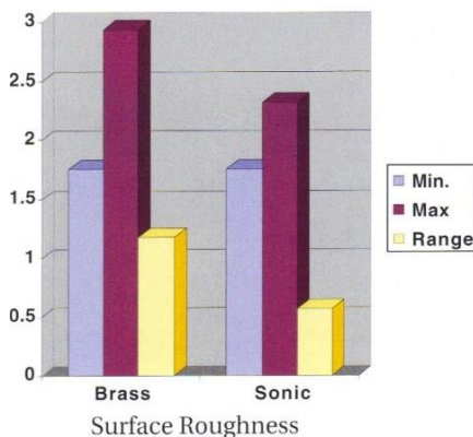
Surface Roughness
